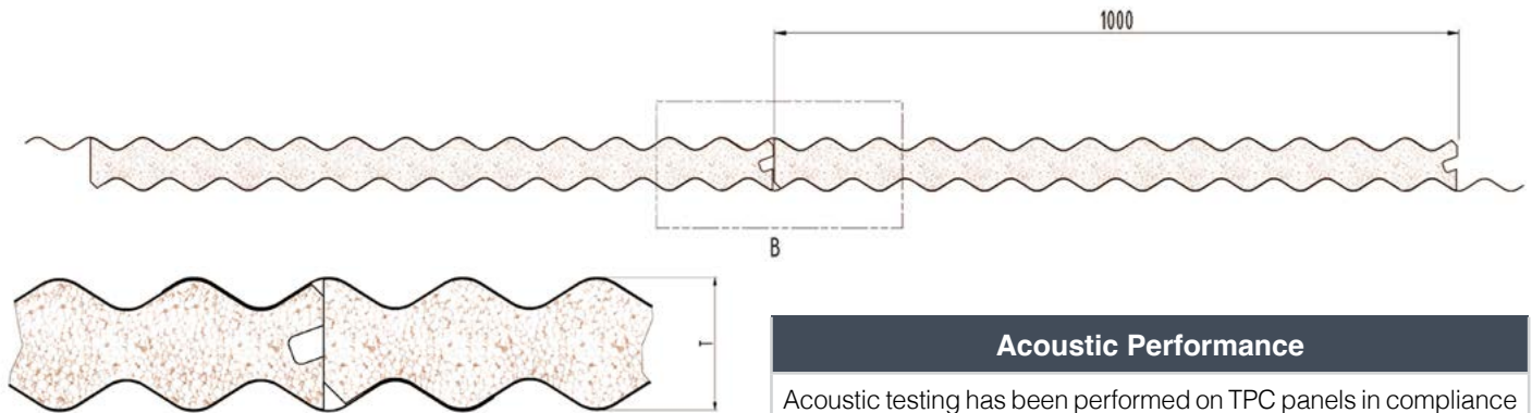
Detail B
