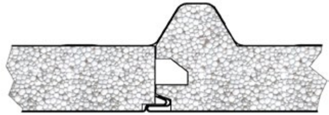
Detail A
